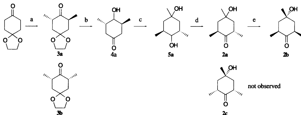
Scheme 1. Reagents and conditions: (a) 1. LDA, MeI, THF:HMPA (3:1) -40^{\circ}\text{C} ; 2. LDA, MeI THF:HMPA (3:1) -78^{\circ}\text{C} , 48%; (b) 1. \text{NaBH}_4 , MeOH; 2. HCl, MeOH; (c) MeLi, THF, -12^{\circ}\text{C} ; (d) PCC, \text{CH}_2\text{Cl}_2 , 80% (four steps); (e) MeONa, MeOH, 100%.
