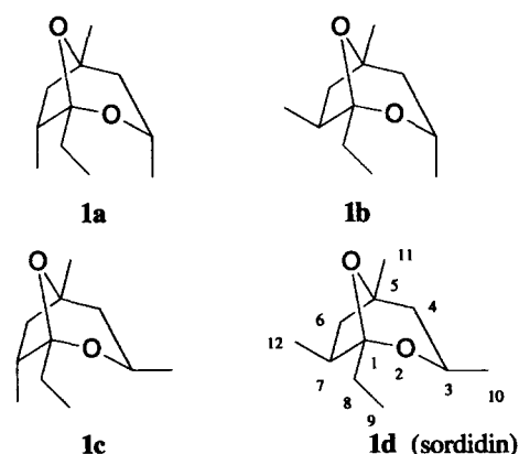
Figure 1. The four stereoisomers of sordidin.
