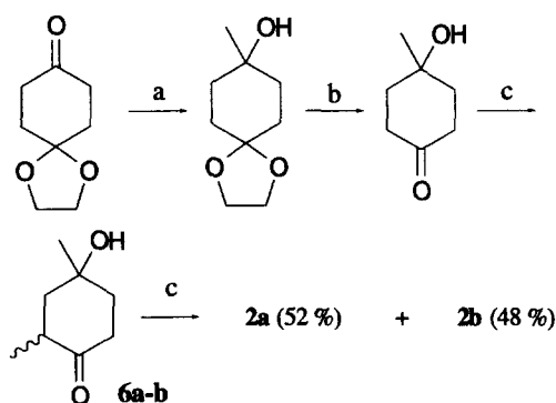
Scheme 2. Reagents and conditions: (a) MeLi, THF -12^\circ\text{C} ; (b) HCl, 1 N, MeOH 40^\circ\text{C} , 63% (two steps); (c) LDA, THF:HMPA (3:1), -78^\circ\text{C} , MeI, 41% (two steps).
