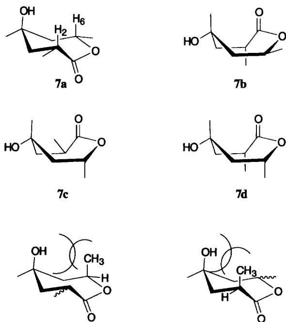
Figure 5. Conformations of lactones 7a–d.
