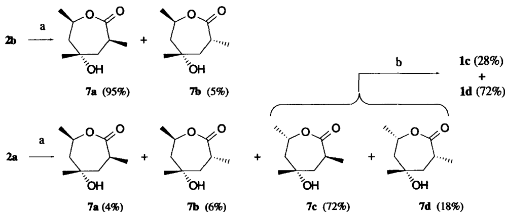
Scheme 3. Reagents and conditions: (a) MCPBA, \text{NaHCO}_3 , \text{CH}_2\text{Cl}_2 (96%); (b) EtLi, pentane (66%).
