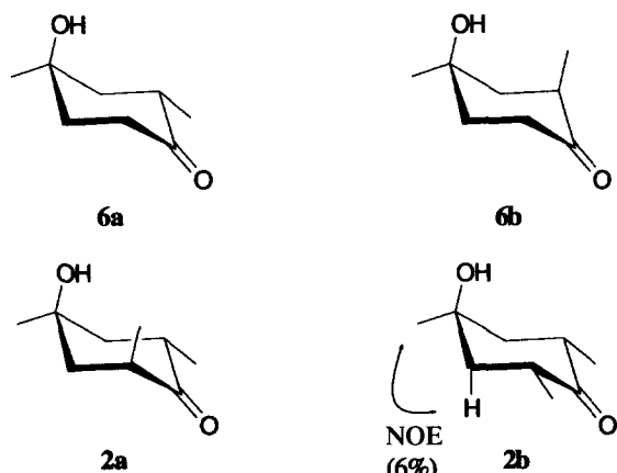
Figure 4. Conformations of 2a and b , and 6a and b .
